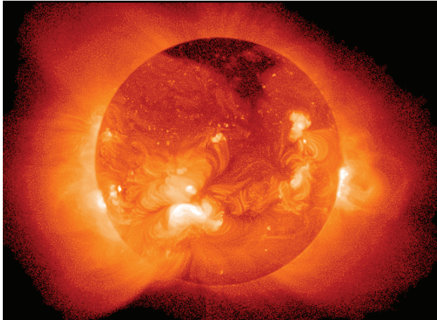
Our Sun produces enormous quantities of helium-3. Particles of helium-3 are sent throughout the solar system by the solar wind. The Moon appears to have substantially more helium-3 than the Earth.
